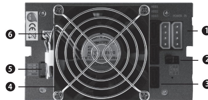
2.4.1 rear view of 2 to 3 canister
